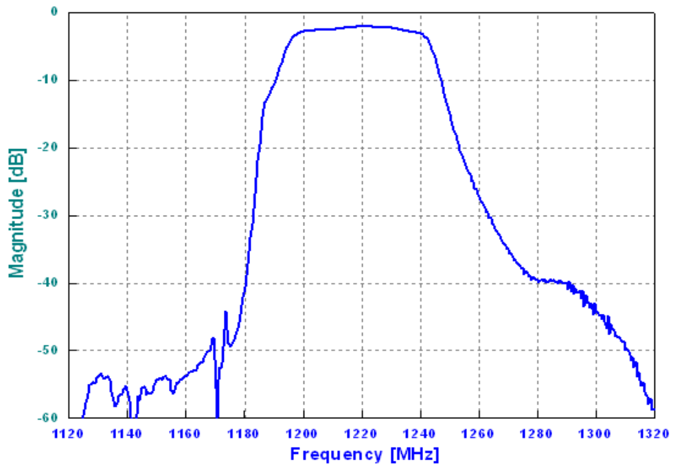
Frequency Response
